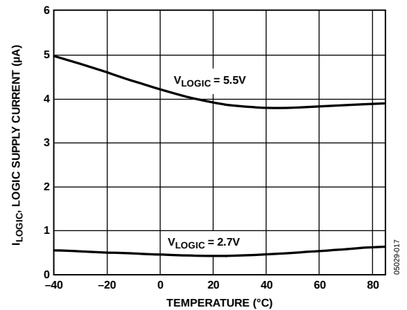
Figure 16. Logic Supply Current vs. Temperature vs. V_{\text{LOGIC}}
