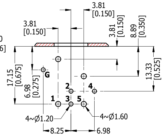
PCB LAYOUT COMPONENT SIDE TOLERANCE: \pm 0.05\text{mm} [.002"]
