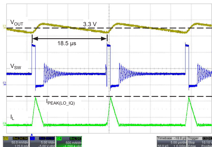
Figure 4: Low-IQ PFM Mode Operation at V_{\text{IN}} = 12 V, V_{\text{OUT}} = 3.3 V, and I_{\text{OUT}} = 66 mA. SW turns on only once every 18.5 \mu\text{s} to regulate V_{\text{OUT}}
