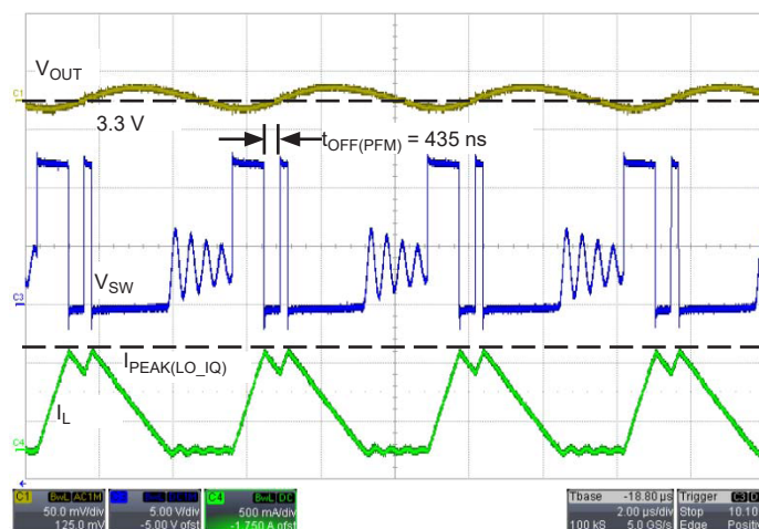
Figure 5: Low-IQ PFM Mode Operation at V_{\text{IN}} = 12 V, V_{\text{OUT}} = 3.3 V, and I_{\text{OUT}} = 330 mA. SW turns on only twice every 5 \mu\text{s} to regulate V_{\text{OUT}}
