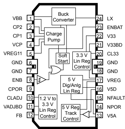
Pinout Diagram
