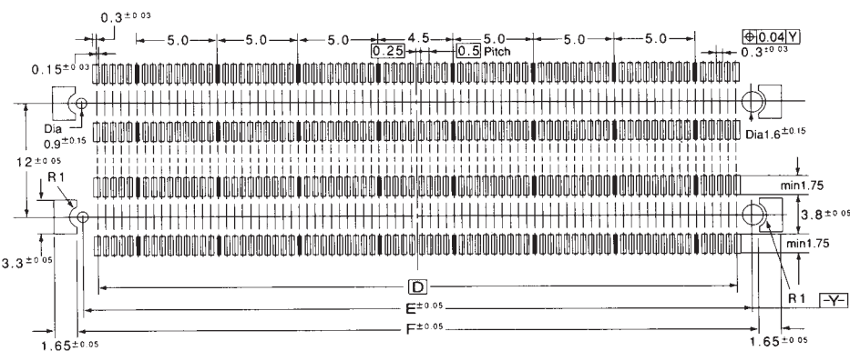
PC Board Layout (|| = For Grounding Contact)
