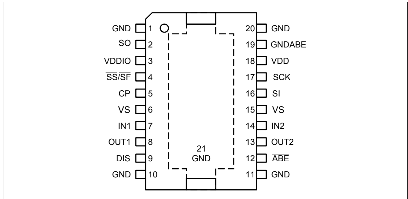
Figure 1 Pinout TLE8209-2SA
