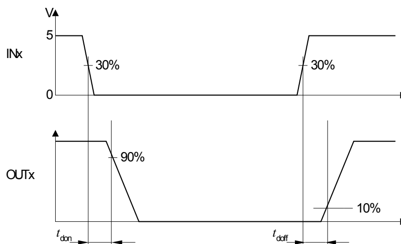
Figure 6 Output Delay Time – Low-Side FETs
