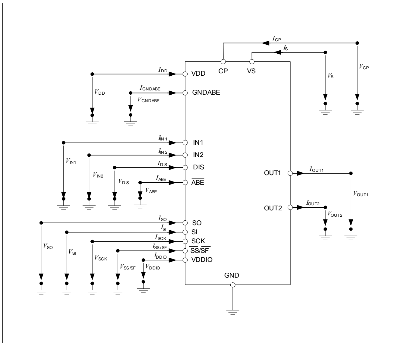
Figure 2 Terms TLE8209-2SA
