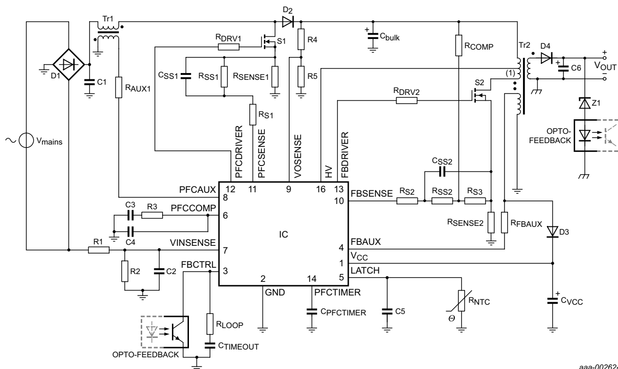
Fig 18. TEA1755LT typical application diagram
