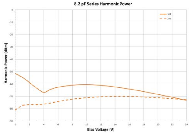
Figure 3. Harmonic Power*
