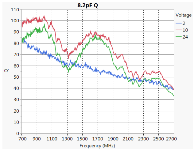
Figure 5. Q*
