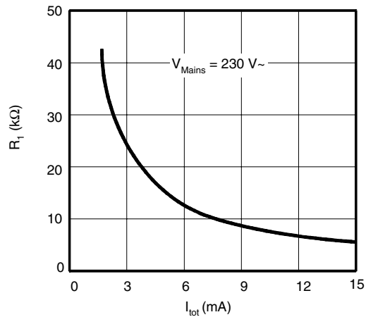
Figure 6-1. Maximum Resistance of R_1
