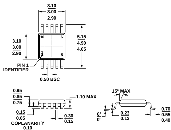
Figure 19. 10-Lead Mini Small Outline Package [MSOP] (RM-10) Dimensions shown in millimeters
