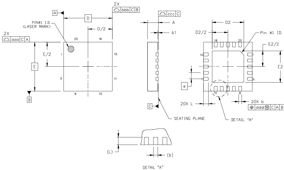
Figure 46. QFN-20 Package
