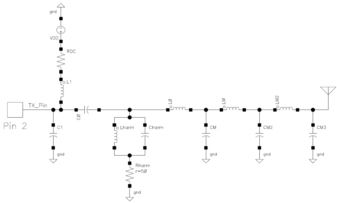
Figure 45. TX Matching and Filtering for Different Bands
