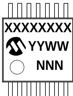
14-Lead TSSOP (4.4 mm)
