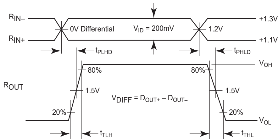
Figure 2. Driver Propagation Delay & Transition Time Waveforms
