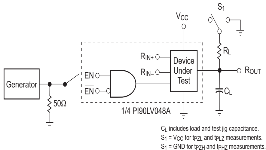
Figure 3. Receiver 3-State Delay Test Circuit
