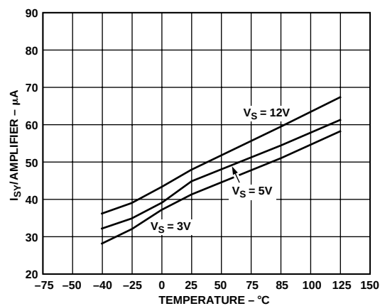
TPC 25. Supply Current/Amplifier vs. Temperature
