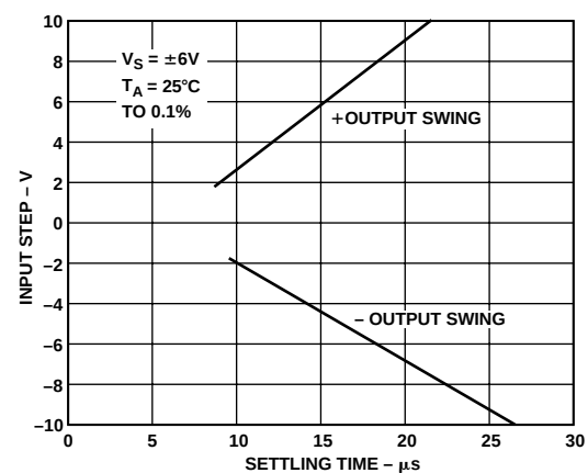
TPC 29. Settling Time to 0.1% vs. Step Size
