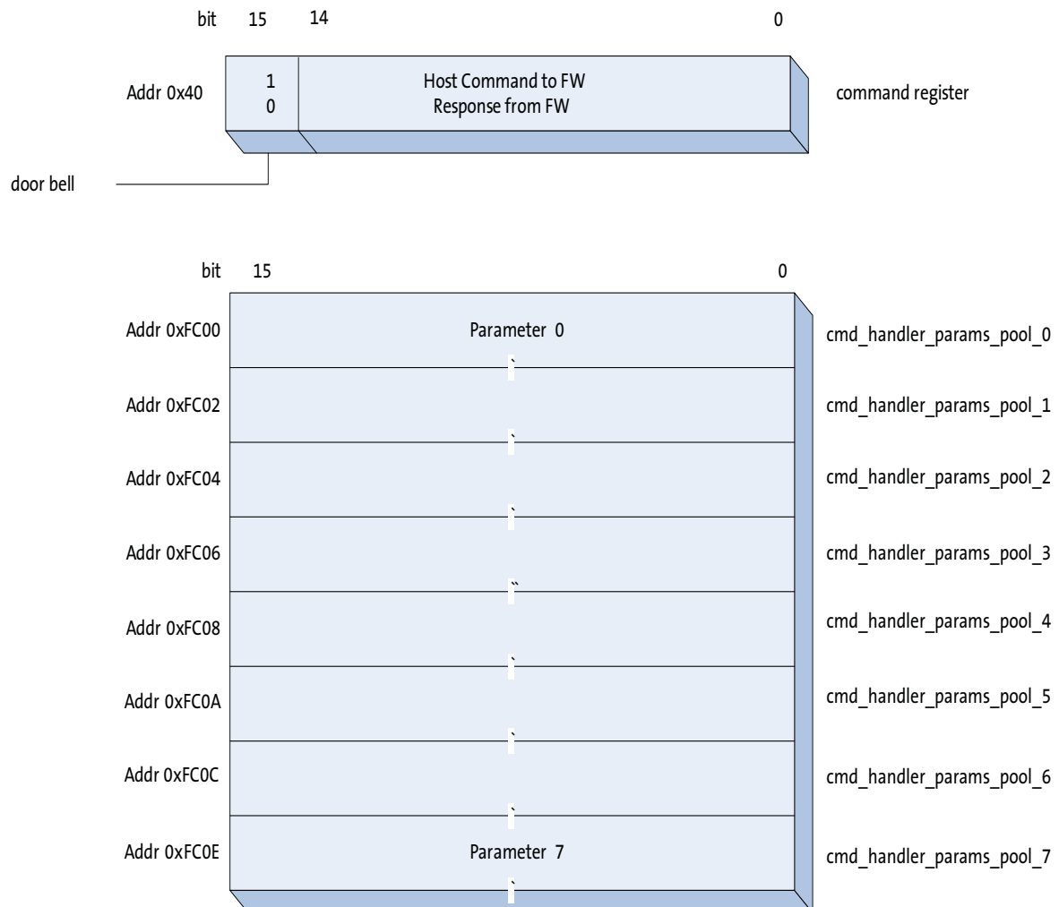
Figure 23: Interface Structure
