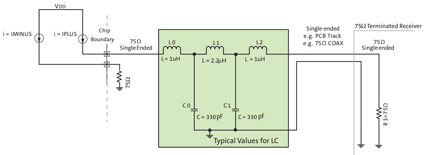
Figure 39: Single-Ended Termination
