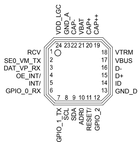
4mm × 4mm 24-pin MLF (ML)
