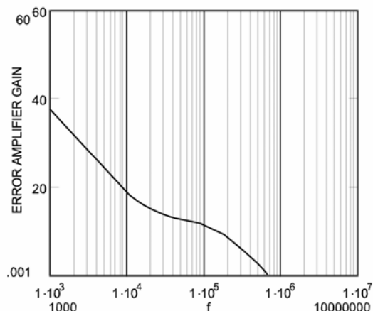
Figure 7. Error Amplifier Gain Curve
