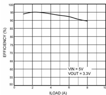
MIC2168A Efficiency
