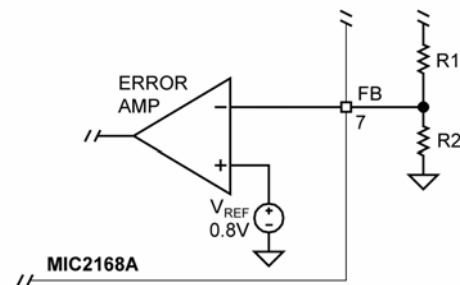
Figure 2. Voltage-Divider Configuration
