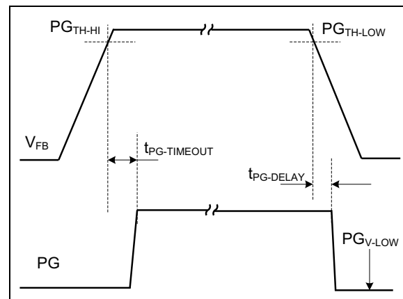
FIGURE 4-2: Power Good Signal.
