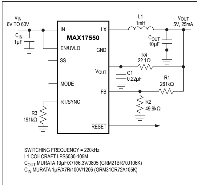
Figure 6. High-Efficiency 5V, 25mA Regulator
