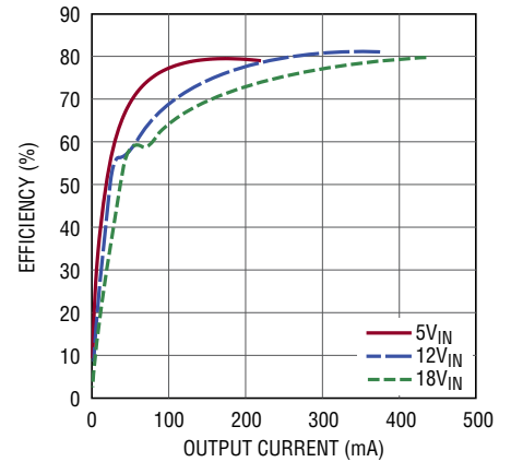
Efficiency -15V OUT Inverting Converter
