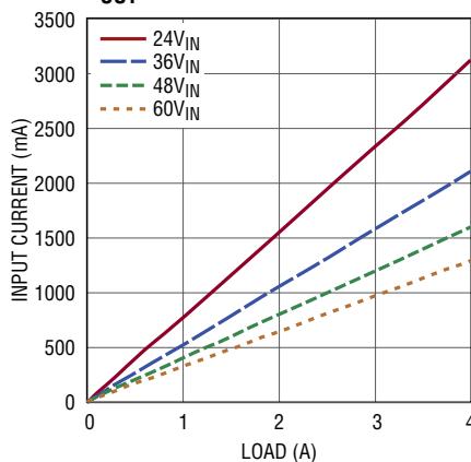
Input Current vs Load, V_{OUT} = 18V
