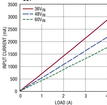
Input Current vs Load, V_{OUT} = 24V
