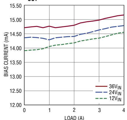
Bias Current vs Load, V_{OUT} = 2.5V
