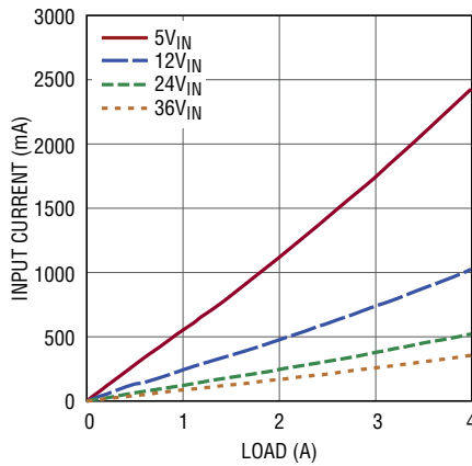
Input Current vs Load, V_{OUT} = 2.5V
