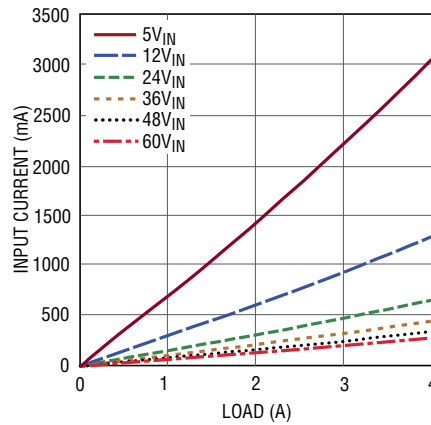
Input Current vs Load, V_{OUT} = 3.3V
