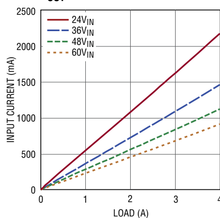
Input Current vs Load, V_{OUT} = 12V
