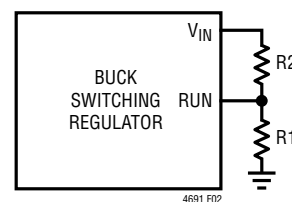
Figure 2. RUN Divider
