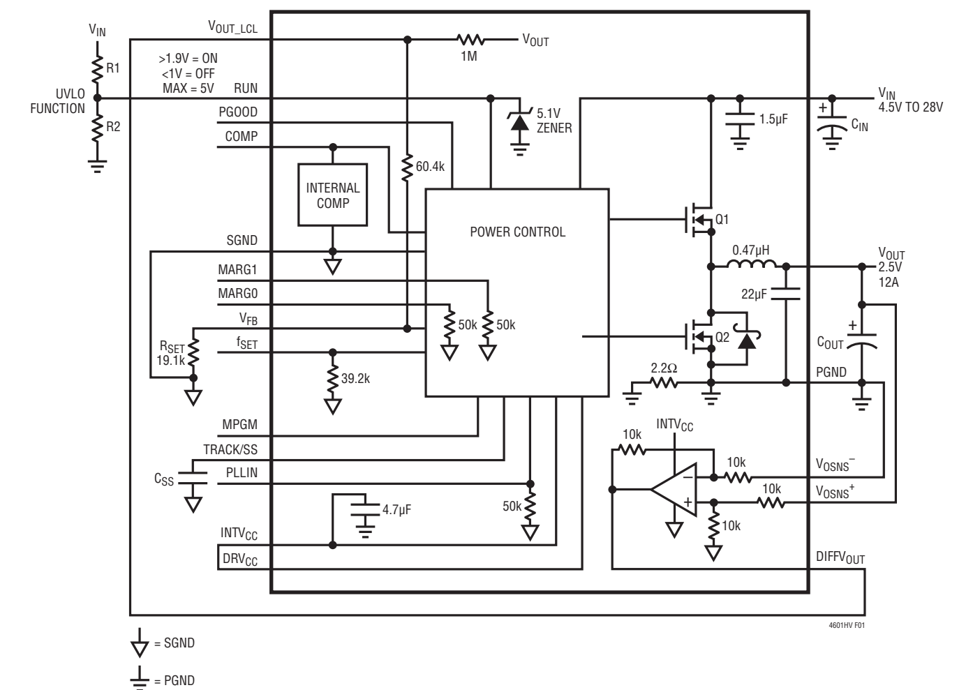
Figure 1. Simplified LTM4601HV Block Diagram
