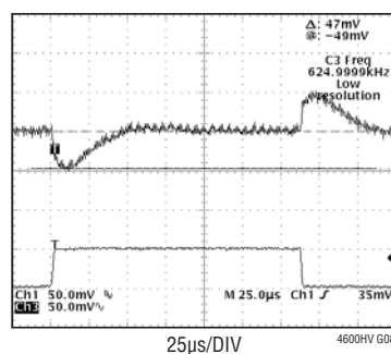
2.5V Transient Response
