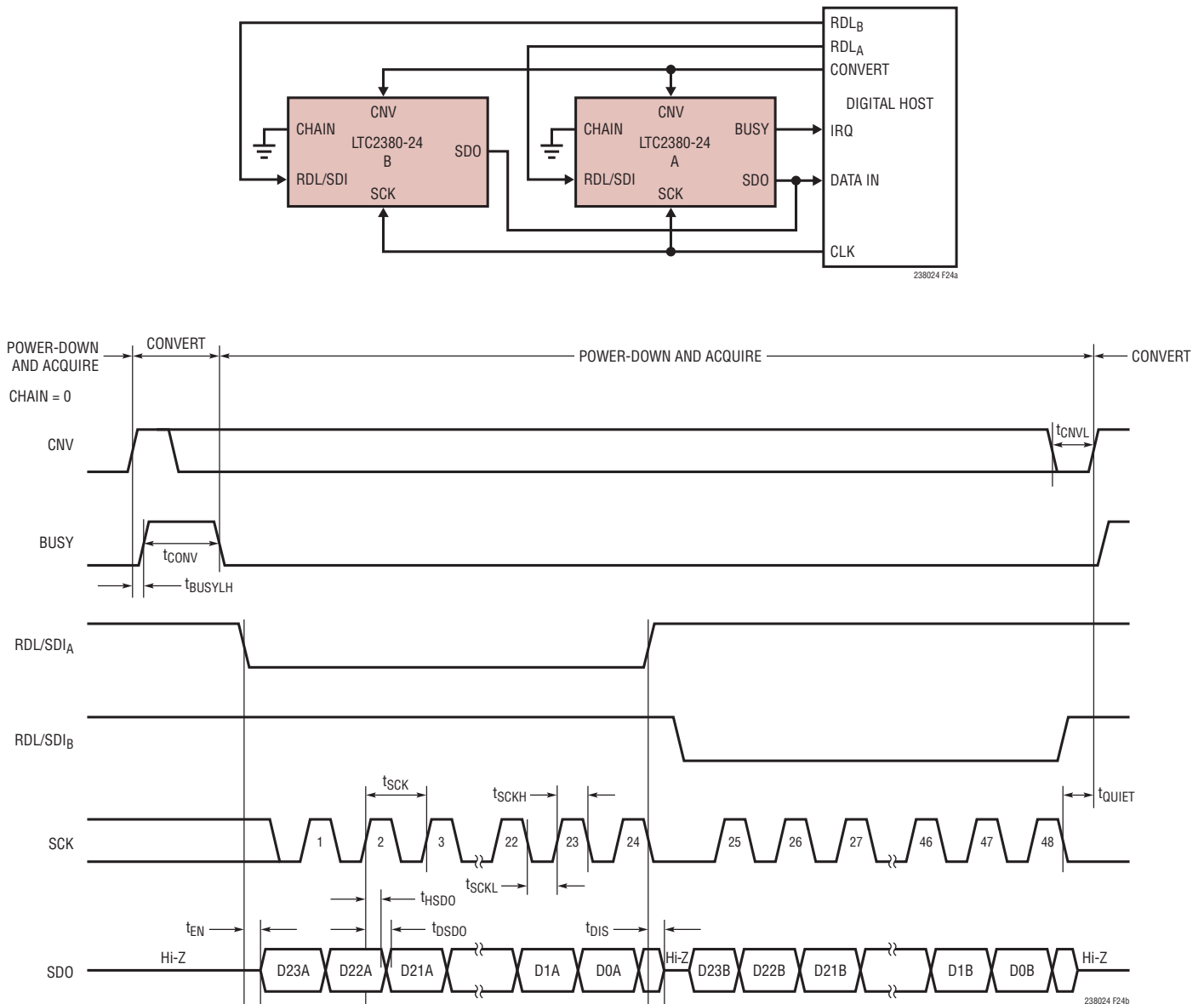
Figure 24. Normal Mode with Multiple Devices Sharing CNV, SCK and SDO
