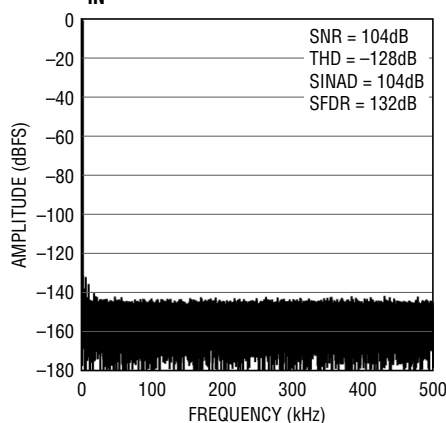
128k Point FFT f_S = 1\text{Mps} , f_{IN} = 2\text{kHz}
