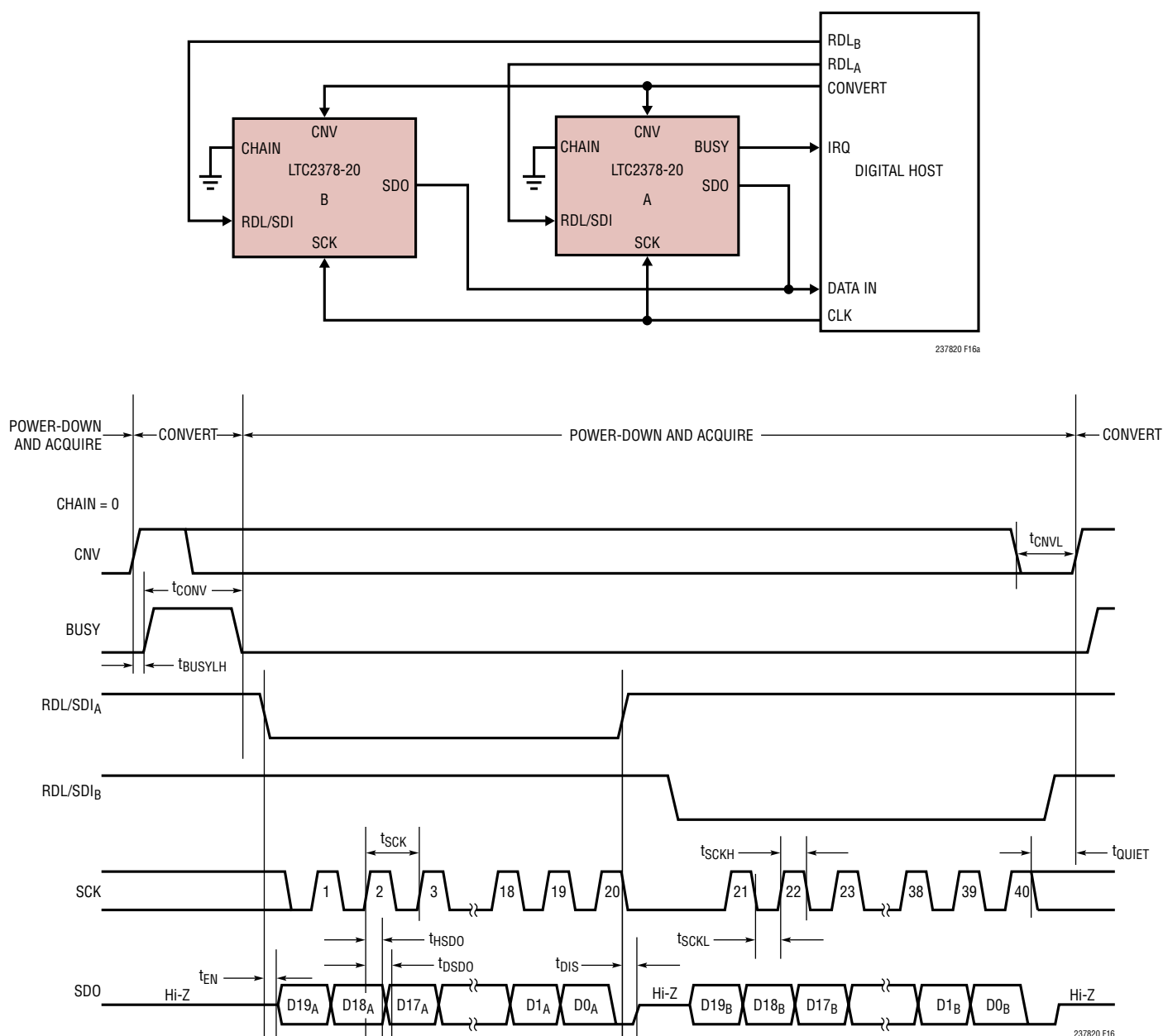
Figure 16. Normal Mode With Multiple Devices Sharing CNV, SCK and SDO
