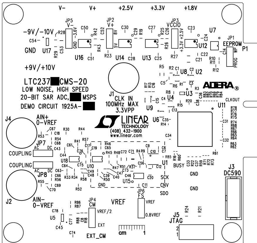
Top Silkscreen
