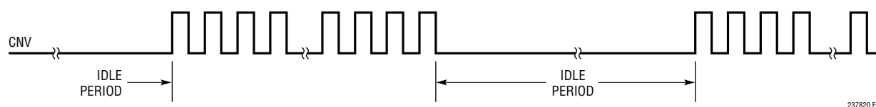
Figure 12. CNV Waveform Showing Burst Sampling
