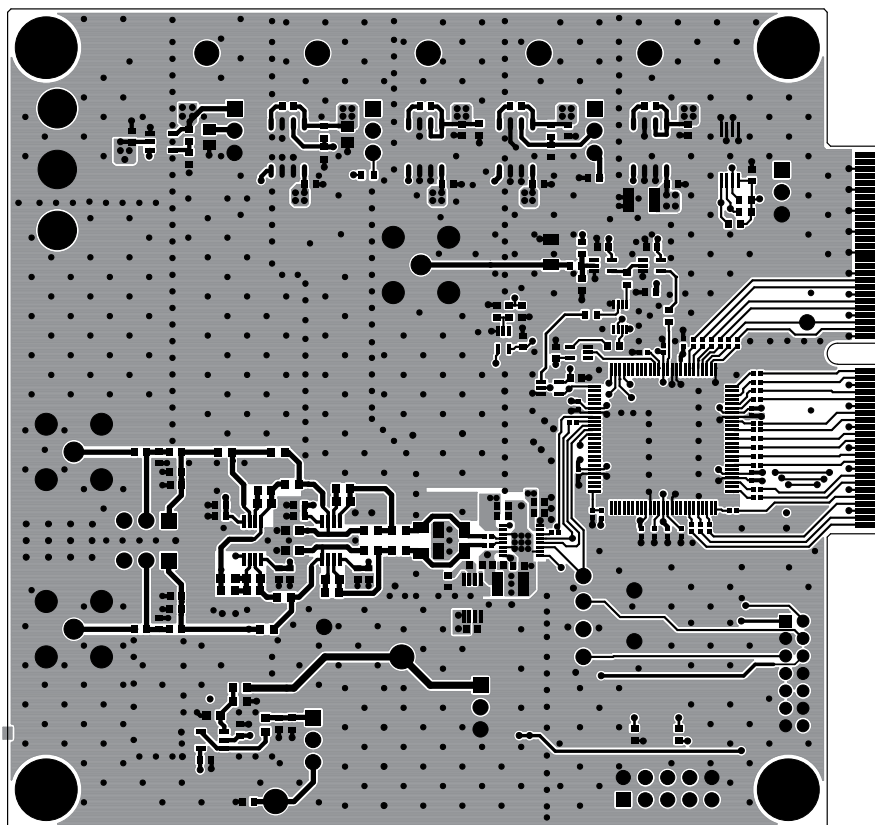
Layer 1 Component Side
