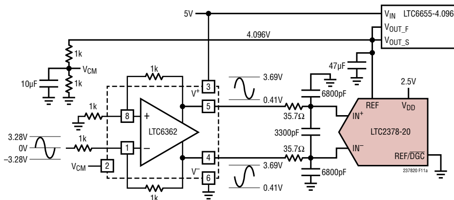
Figure 11a. LTC6362 Configured to Accept a \pm 3.28\text{V} Input Signal While Running from a Single 5V Supply When Digital Gain Compression Is Enabled in the LTC2378-20
