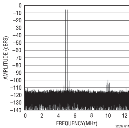
LTC2203: 32K Point 2-Tone FFT, f_{IN} = 4.9\text{MHz} and 30.1\text{MHz} , -7\text{dBFS} , PGA = 0
