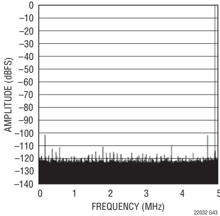
LTC2202: 128K Point FFT, f_{IN} = 5.1\text{MHz} , -1\text{dBFS} , PGA = 0
