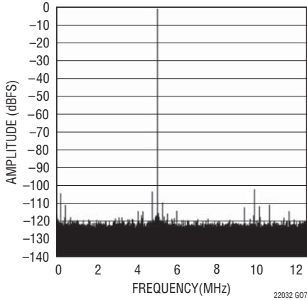
LTC2203: 128K Point FFT, f_{IN} = 5.1\text{MHz} , -1\text{dBFS} , PGA = 0
