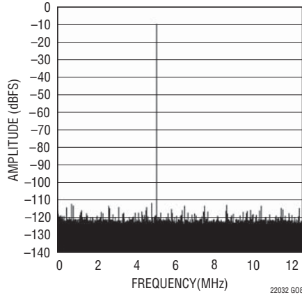
LTC2203: 128K Point FFT, f_{IN} = 5.1\text{MHz} , -10\text{dBFS} , PGA = 0
