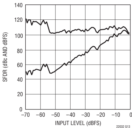
LTC2203: SFDR vs Input Level, f_{IN} = 5\text{MHz} , PGA = 0, Dither "Off"
