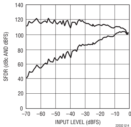
LTC2203: SFDR vs Input Level, f_{IN} = 5\text{MHz} , PGA = 0, Dither "On"
