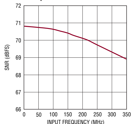
LTC2171-12: SNR vs Input Frequency, -1\text{dBFS} , 2\text{V} Range, 40\text{MSPS}
