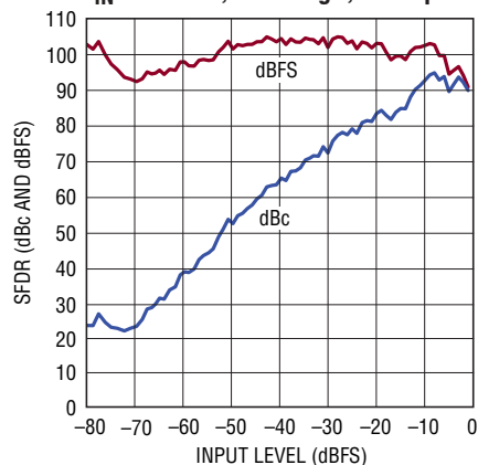
LTC2171-12: SFDR vs Input Level, f_{IN} = 70\text{MHz} , 2\text{V} Range, 40\text{MSPS}
