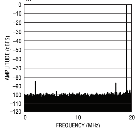
LTC2171-12: 8k Point FFT, f_{IN} = 139\text{MHz} , -1\text{dBFS} , 40\text{MSPS}
