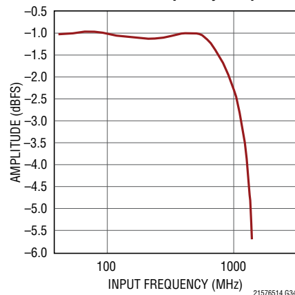
LTC2156-14: Frequency Response
