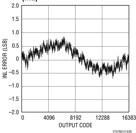
LTC2155-14: Integral Nonlinearity (INL)
