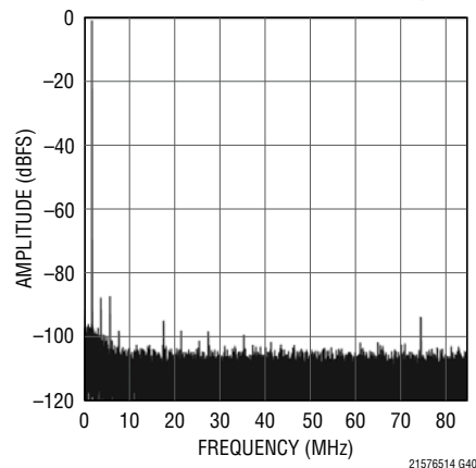
LTC2155-14: 32K Point FFT, f_{IN} = 169\text{MHz} , -1dBFS, 170MSPS
