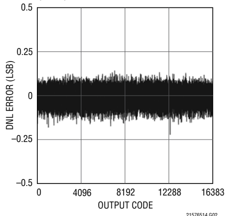
LTC2157-14: Differential Nonlinearity (DNL)
