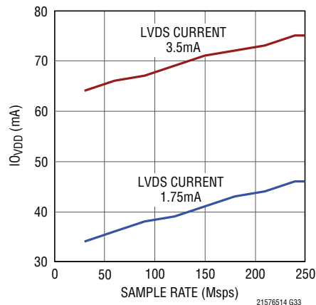
LTC2156-14: I_{OVD} vs Sample Rate, 15MHz Sine Wave Input, -1dBFS
