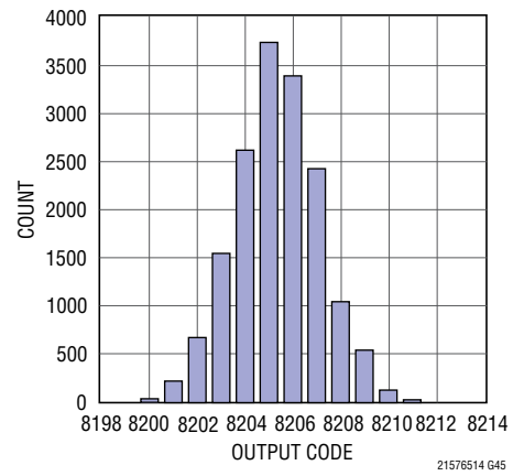
LTC2155-14: Shorted Input Histogram
