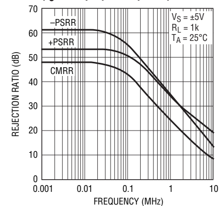
CMRR and PSRR vs Frequency ( I_S = 300\mu A per Amplifier)
