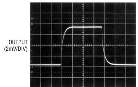
Large-Signal Transient Response ( I_S = 300\mu\text{A} per Amplifier)
