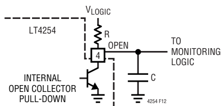
Figure 12. Delay Circuit for OPEN FET Detection
