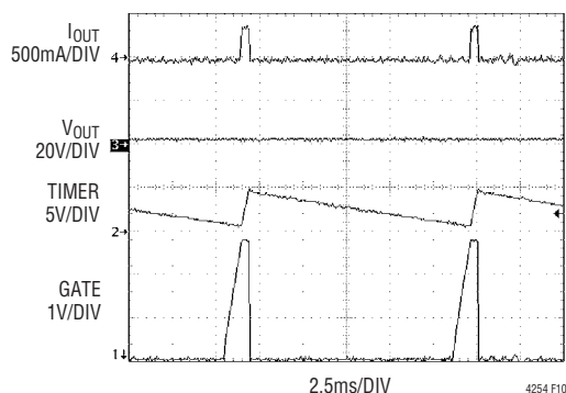
Figure 10. RETRY Waveforms
