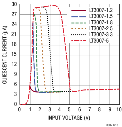
Quiescent Current
