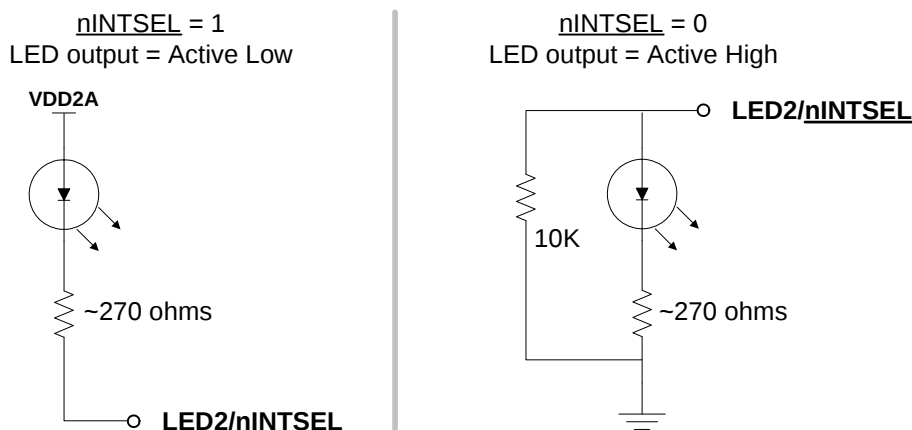
Figure 3.11 \text{LED2}/\overline{\text{nINTSEL}} Polarity Configuration
