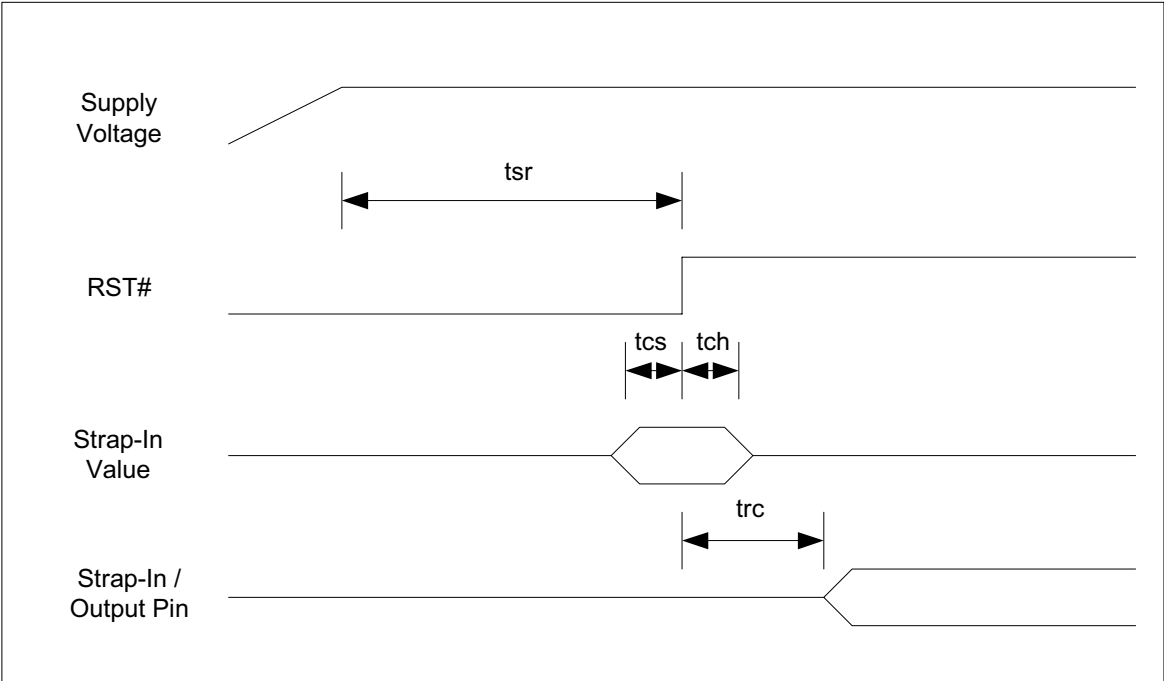
Figure 22. Reset Timing
