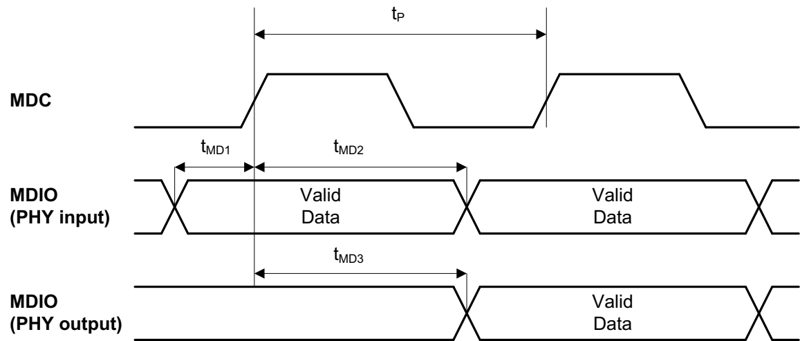
Figure 21. MDC/MDIO Timing
