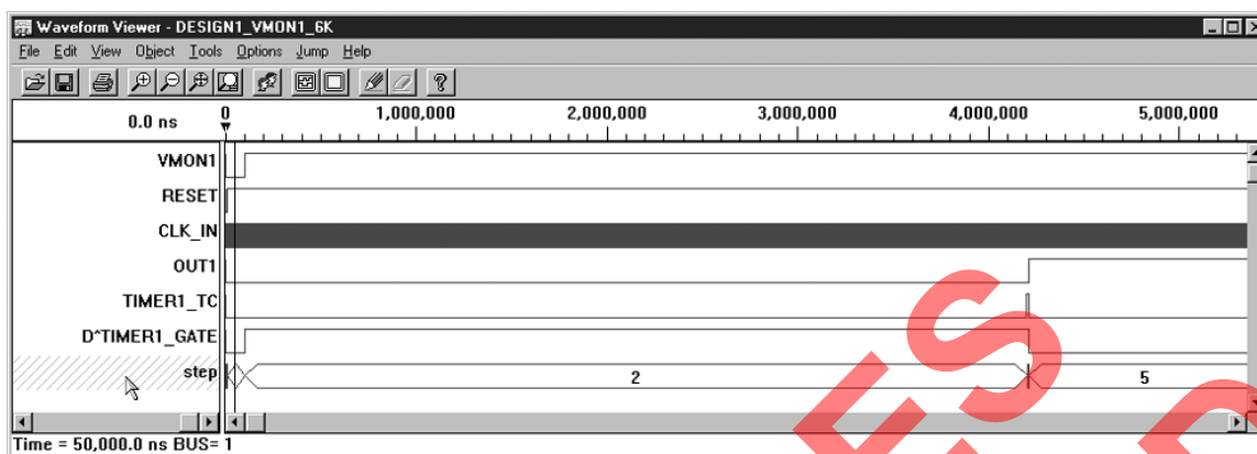
Figure 2-16. PAC-Designer Functional Simulation Screen
