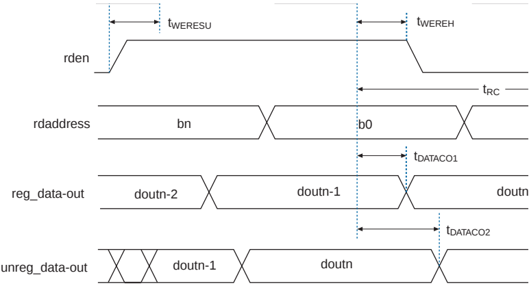
Figure 6–5. Stratix GX Transceiver Reset & PLL Lock Time Waveform Note (1)
