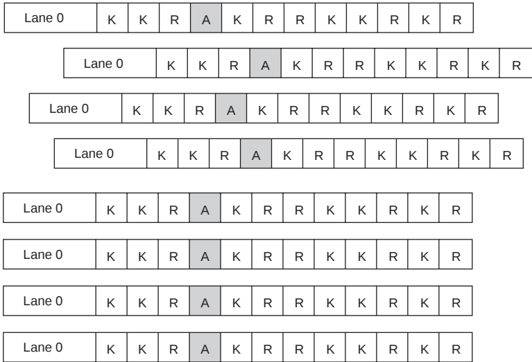
Figure 2–19. Before & After the Channel Aligner
