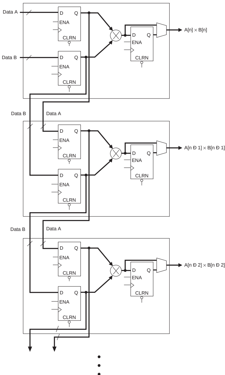
Figure 4–32. Multiplier Sub-Blocks Using Input Shift Register Connections
