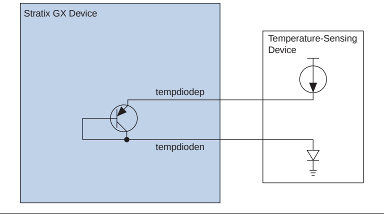
Figure 5–4. External Temperature-Sensing Diode
