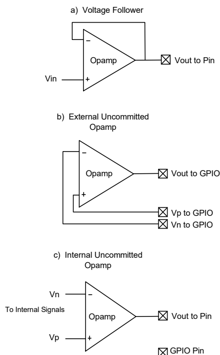
Figure 8-7. Opamp Configurations
