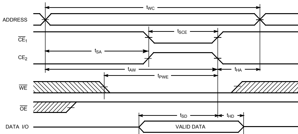
Figure 7. Write Cycle No. 2 ( \overline{\text{CE}}_1 or \overline{\text{CE}}_2 Controlled) [23, 24, 25]
