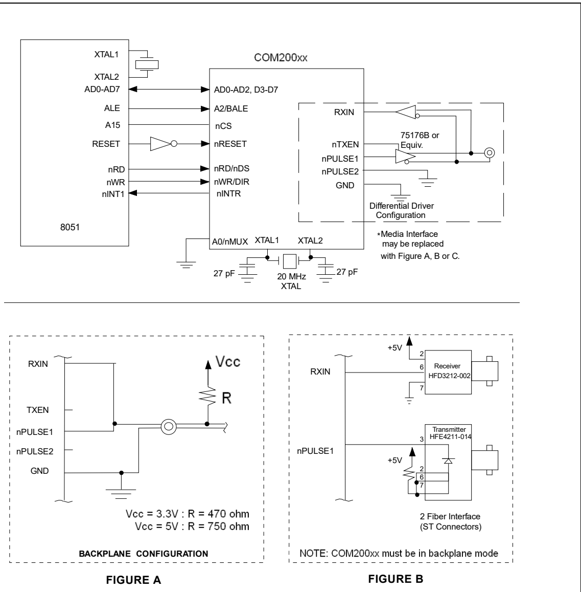
FIGURE 5-1: MULTIPLEXED, 8051-LIKE BUS INTERFACE WITH RS-485 INTERFACE
