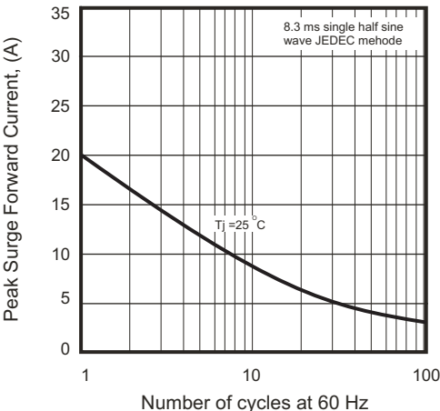
Fig.4 - Non Repetitive Peak Forward Surge Current
