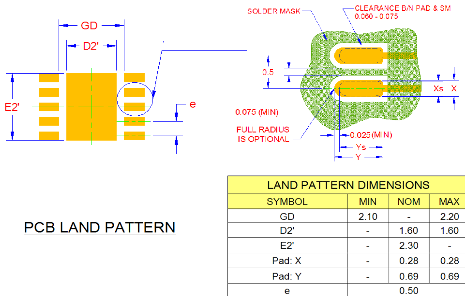
Figure 3 10-Pin DFN 3mm x 3mm PCB Footprint
