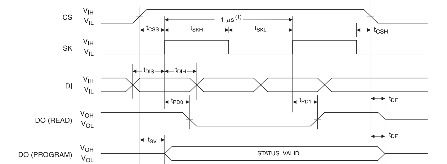
Figure 2. Synchronous Data Timing
