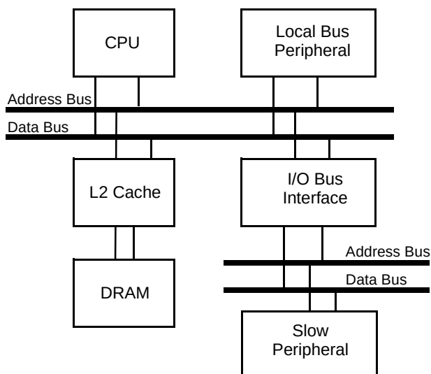
Figure 3. Typical System Block Diagram for \text{HOLD}/\text{HLDA} Bus Arbitration
