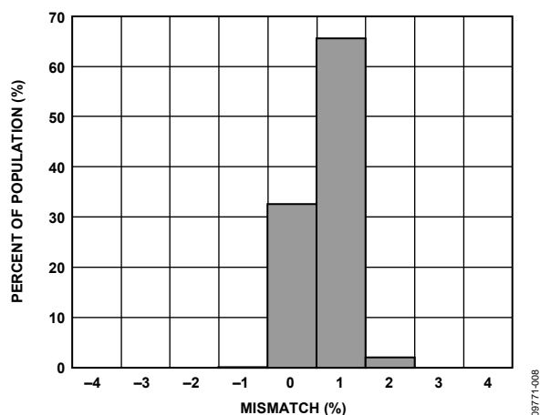
Figure 12. Self-Test Mismatch at 25°C
