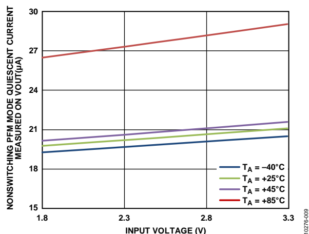
Figure 11. ADP1607 Nonswitching PFM Mode Quiescent Current Measured on VOUT vs. Input Voltage
