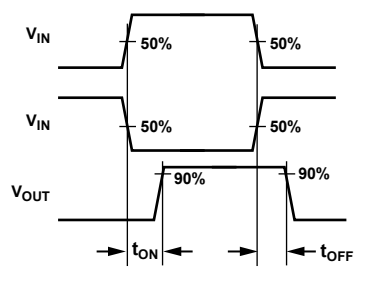
Figure 29. Switching Timing
