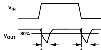
Figure 30. Break-Before-Make Delay, t_D
