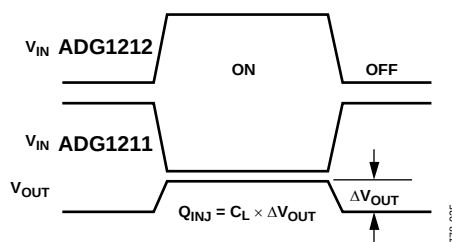
Figure 25. Charge Injection
