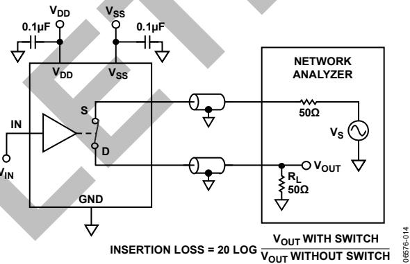
Figure 24. Bandwidth
