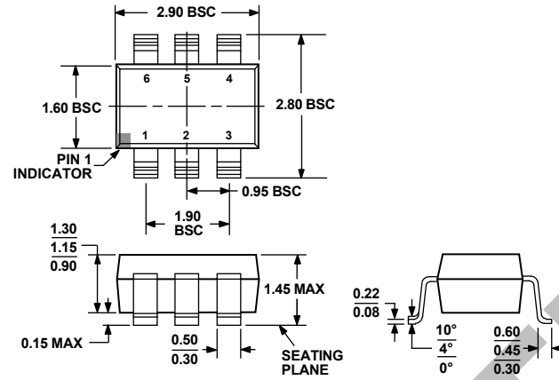
Figure 28. 6-Lead Small Outline Transistor Package [SOT-23] (RJ-6)
