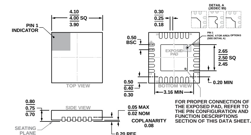
Figure 79. 24-Lead Lead Frame Chip Scale Package (LFCSP) 4 mm × 4 mm Body and 0.75 mm Package Height (CP-24-7)
