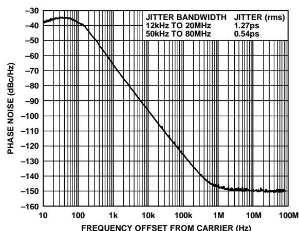
Figure 8. Phase Noise, Pin Programmed ( f_{REF} = 8 kHz, f_{OUT1} = 155.52 MHz)
