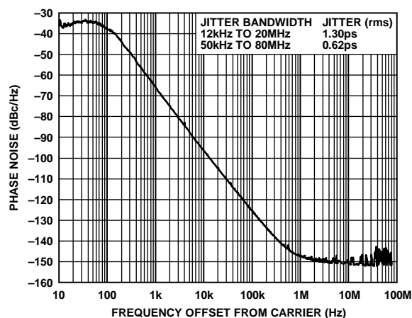
Figure 3. Phase Noise, Pin Programmed ( f_{XTAL} = 25 MHz, f_{OUT1} = 156.25 MHz)
