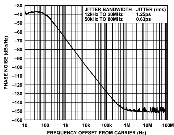
Figure 5. Phase Noise, Pin Programmed ( f_{REF} = 61.44 MHz, f_{OUT1} = 122.88 MHz)
