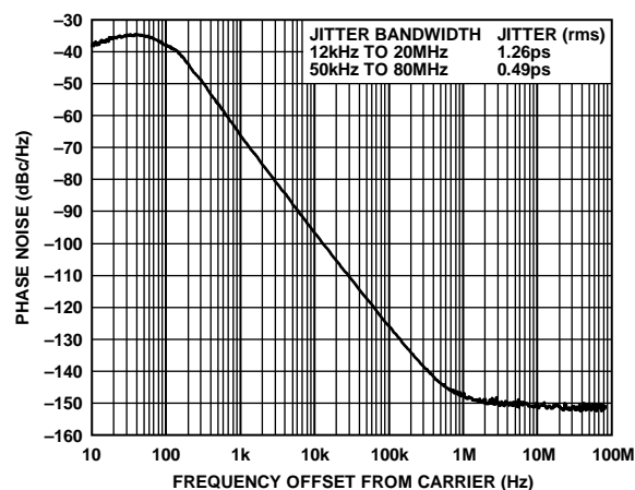
Figure 7. Phase Noise, Pin Programmed ( f_{REF} = 19.44 MHz, f_{OUT1} = 155.52 MHz)
