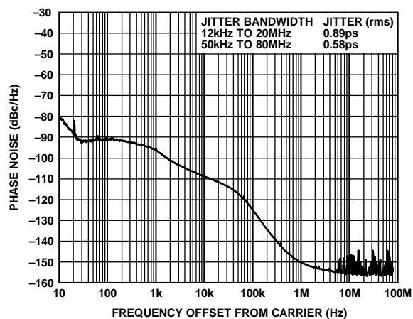
Figure 4. Phase Noise, Pin Programmed ( f_{REF} = 25 MHz, f_{OUT1} = 125 MHz, Pin Ax = 1110)
