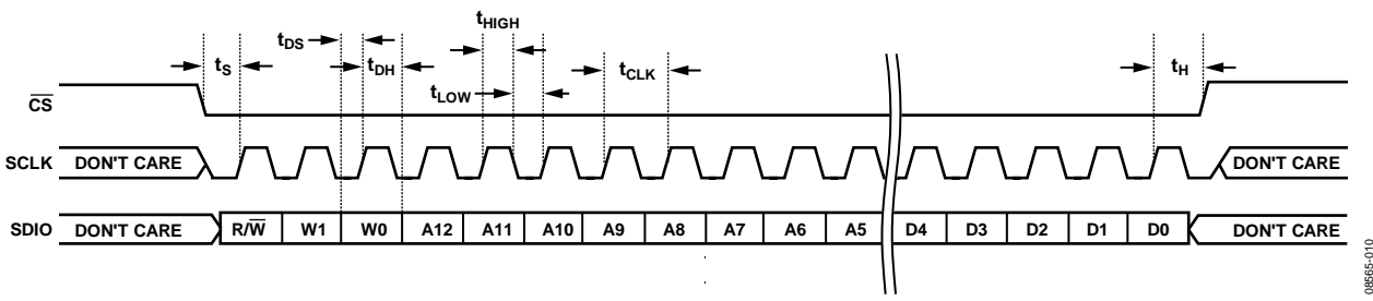
Figure 38. Serial Control Port Write—MSB First, 16-Bit Instruction, Timing Measurements
