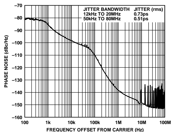
Figure 6. Phase Noise, Pin Programmed ( f_{REF} = 77.76 MHz, f_{OUT1} = 622.08 MHz)
